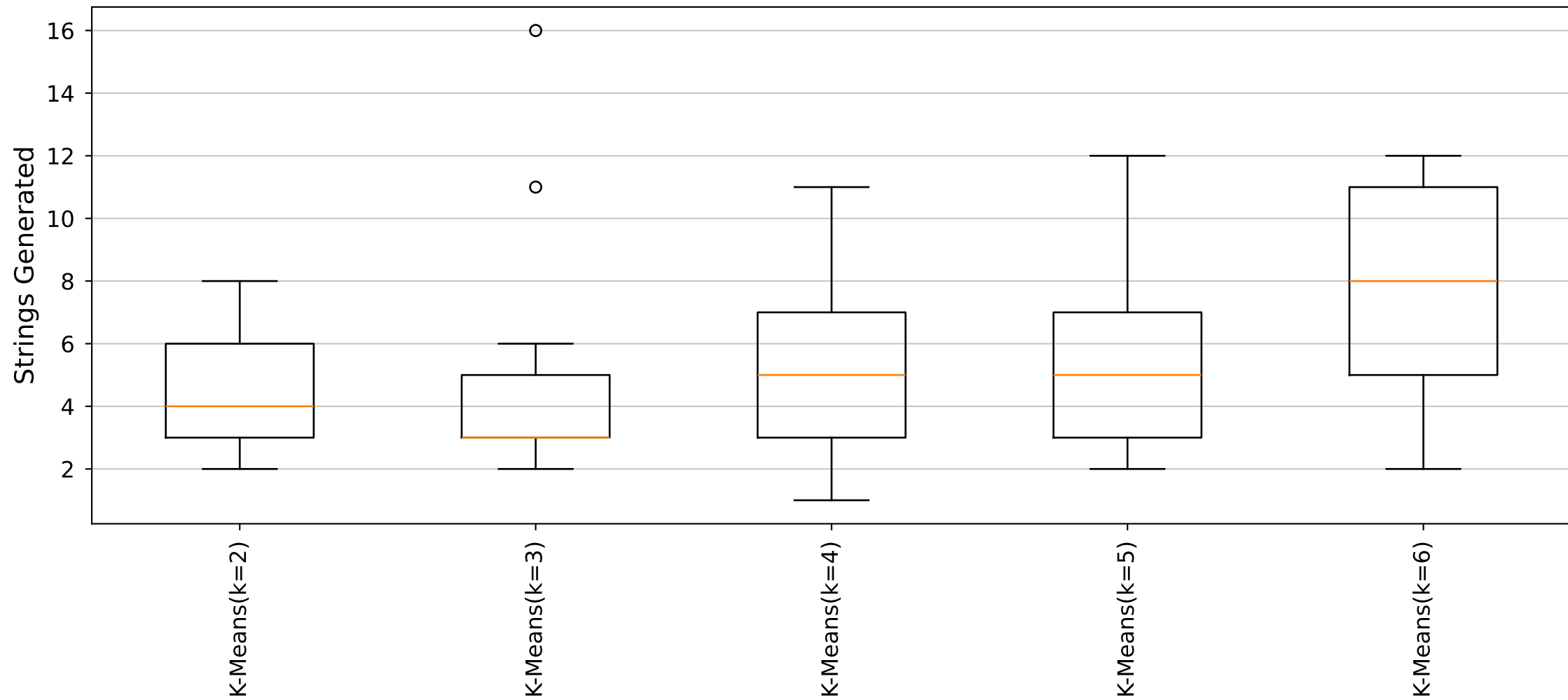
YARA Rules Strings Generated Distribution (Cluster29_Size6 dataset)
